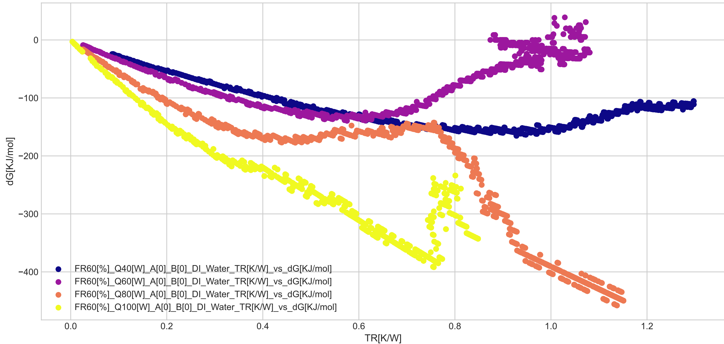
FR [60]% - Q [ 40 60 80 100]W - alpha [0] - beta [0] - DI_Water
